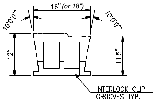
BASIC UNIT "A" (PLAN VIEW)
