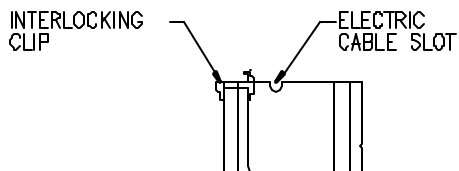
BASIC UNIT "B" SPLITTABLE INTO 8 INCH HALVES (PLAN VIEW)
