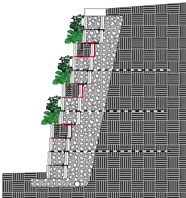
NatureWall, Section View, Detail
