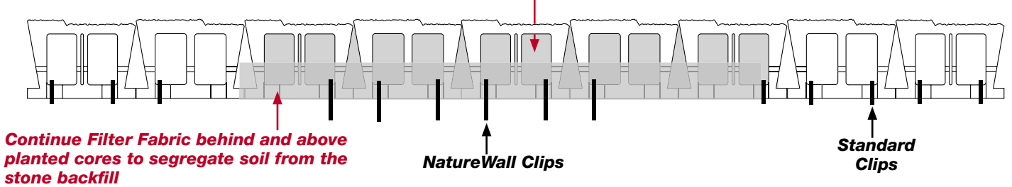
Plan View of StoneWall SELECT retaining wall with NatureWall terraced section in a straight wall, similar to photo above
