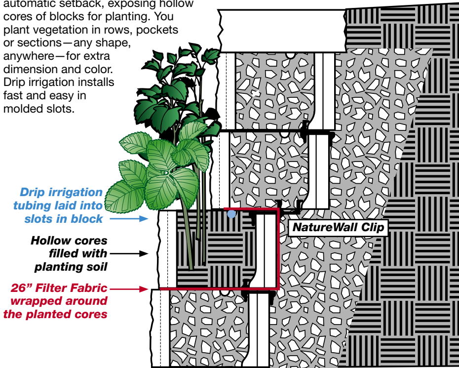
NatureWall, Section View, Detail
